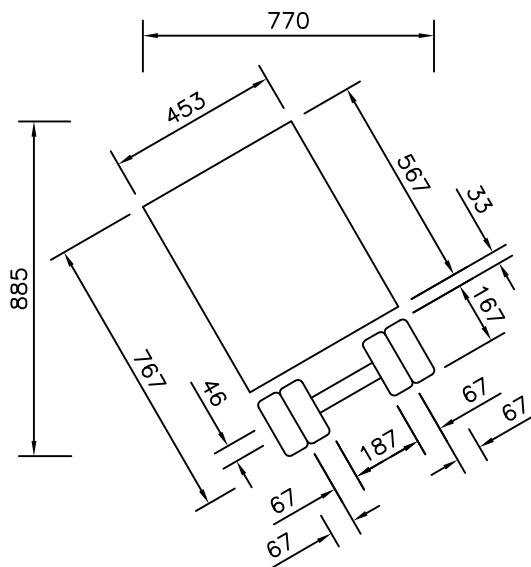
TRUCK DETAILS
