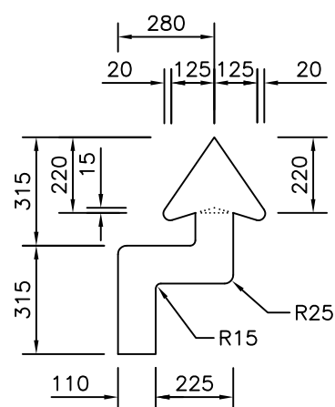
ARROW DETAILS
